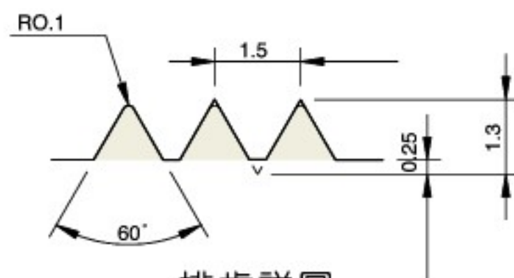
排齒詳圖 Drawing of Serration
