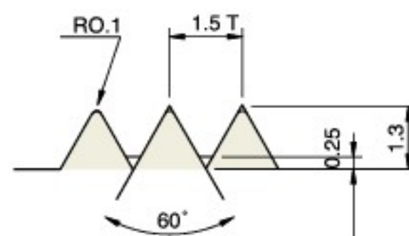
排齒詳圖 Drawing of Serration
